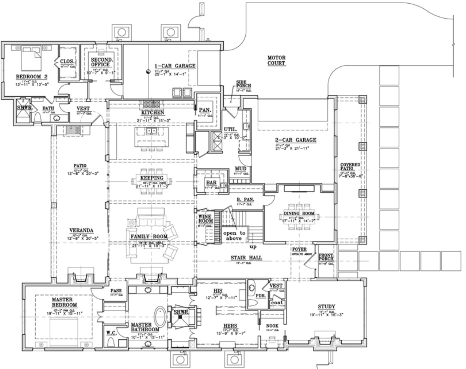
FIRST FLOOR
