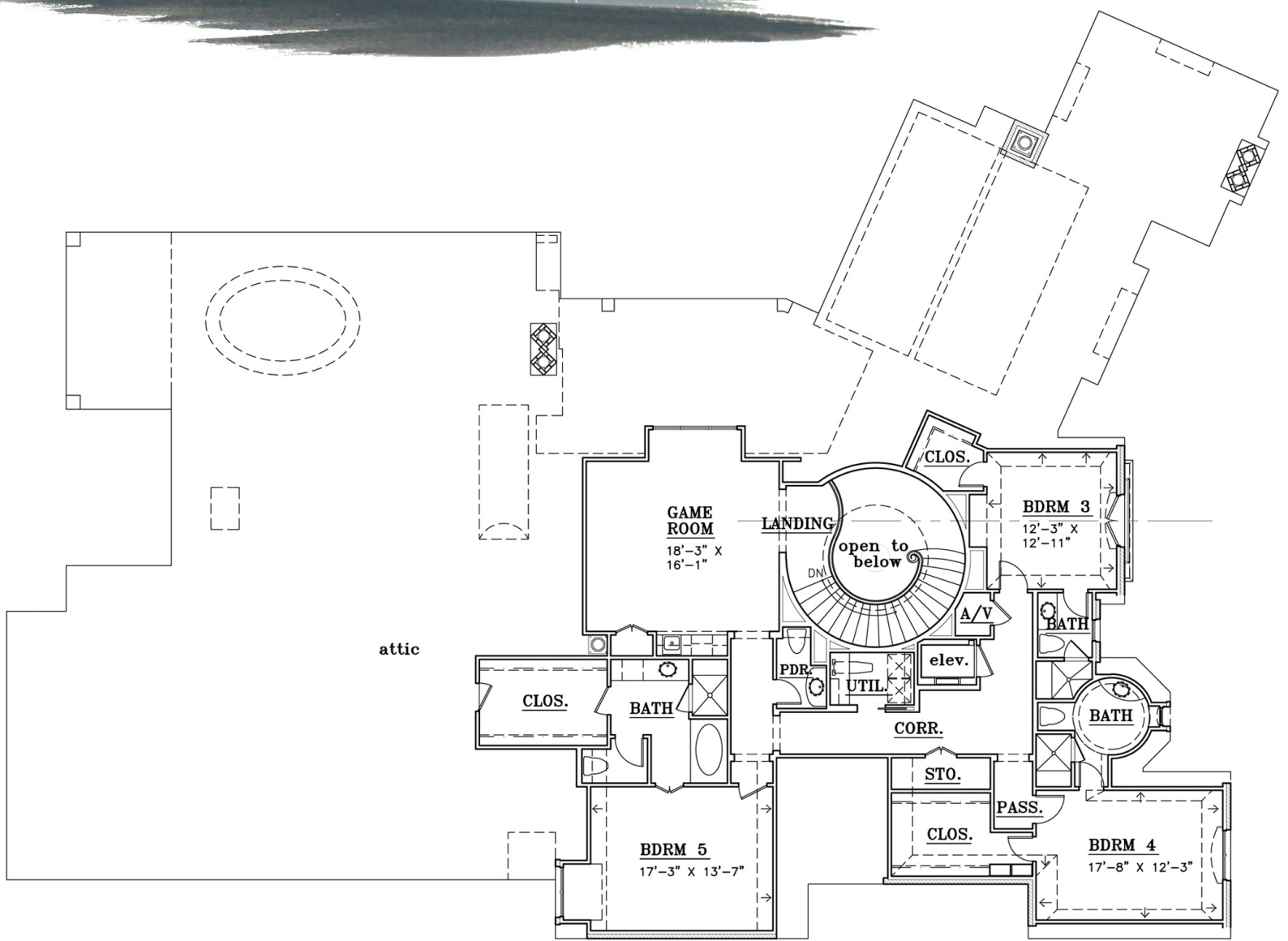
SECOND FLOOR
